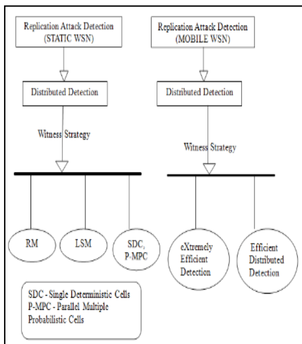
Fig. 2 : Steps of replication attack detection
